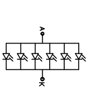
BACKLIGHT CIRCUIT 6 WHITE LED, If=120mA, Vf=32V
