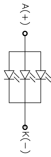
LED CIRCUIT DIAGRAM
